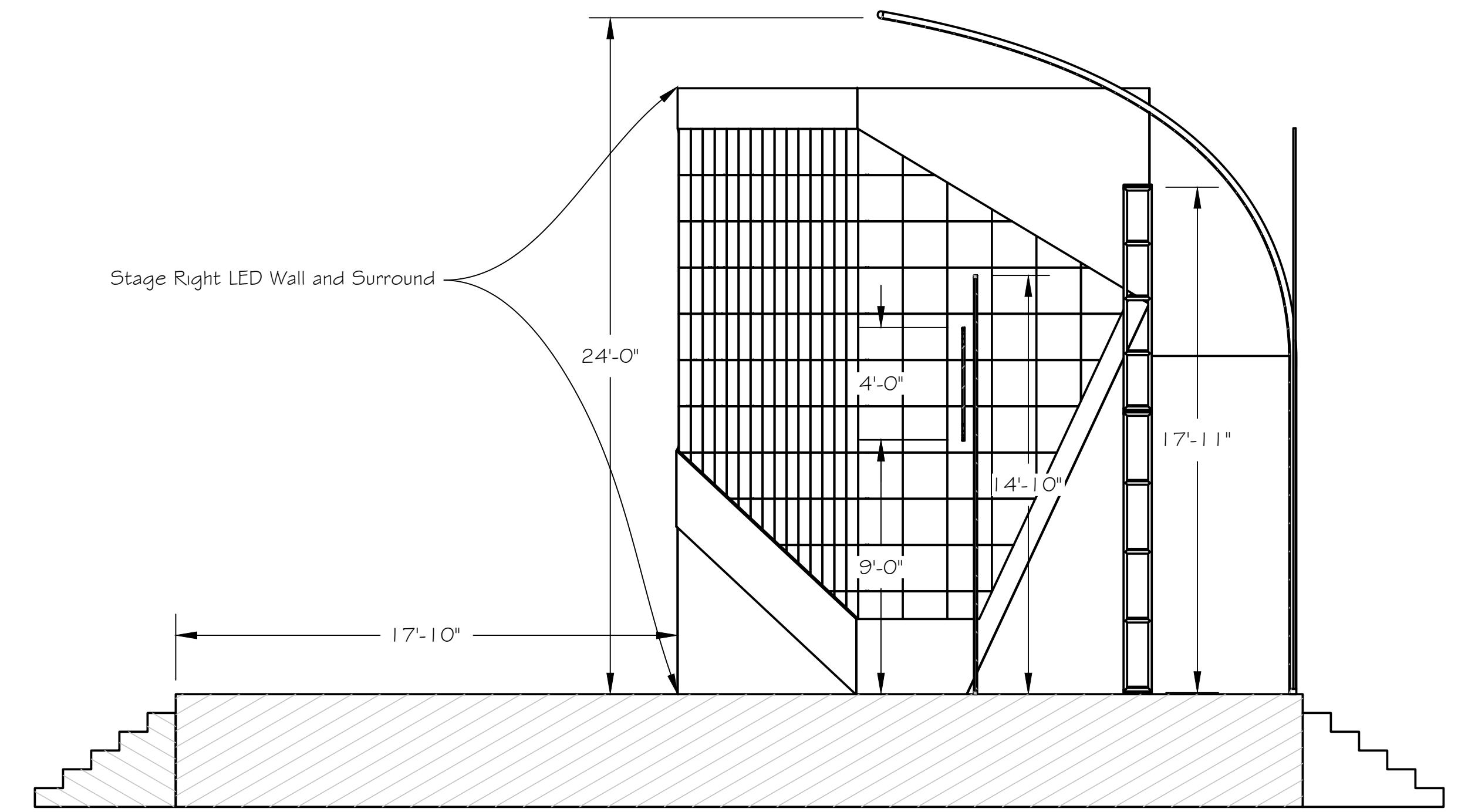
SECTION A-A SCALE 1/4" = 1'-0"
