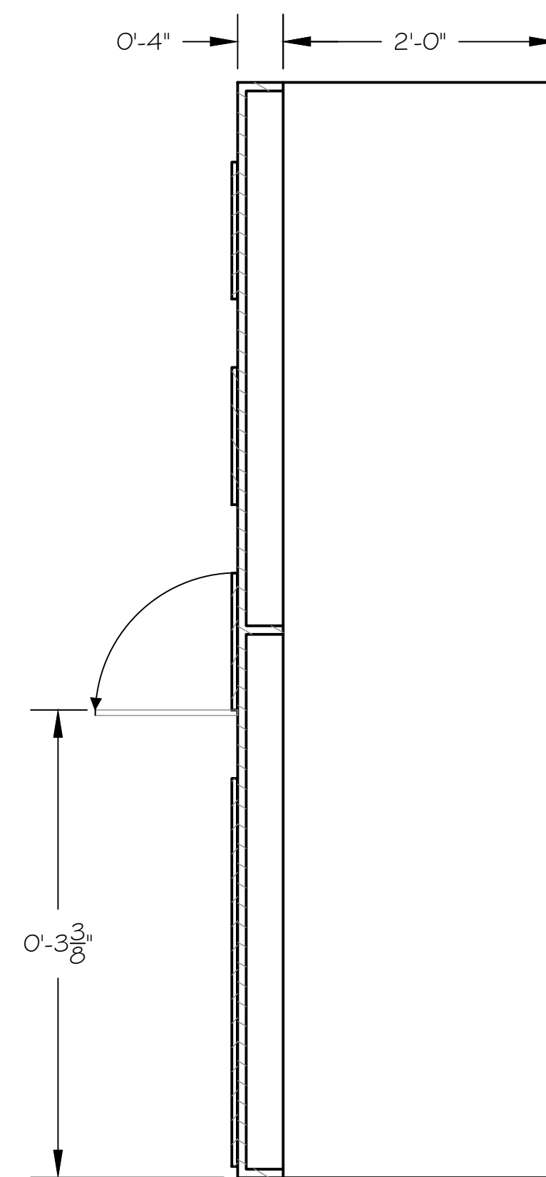
SECTION E-E SCALE 1" = 1'-0"
